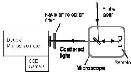
Fig.1 Raman scattering setup
