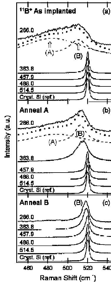
Fig.3 Raman spectra of as-implanted Si (a), and after annealing A (b) and B (c) for five different excitation laser wavelengths (nm).
