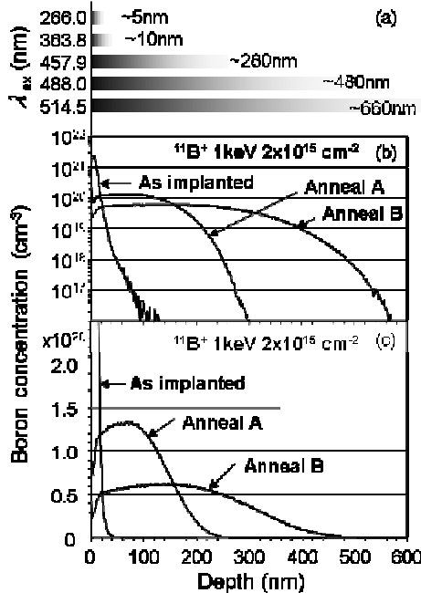
Fig.2 Laser penetration depth (a) and SIMS depth profile of boron in logarithmic (b) and linear scale (c).
